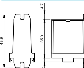
Rear flange mount adaptor for 55.32, 55.33, 55.34
