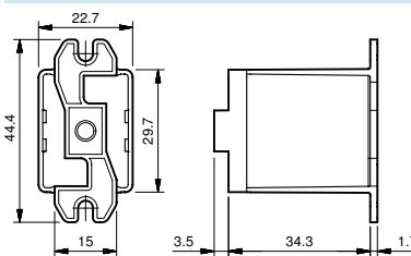
Top flange mount adaptor for 55.32, 55.33, 55.34
